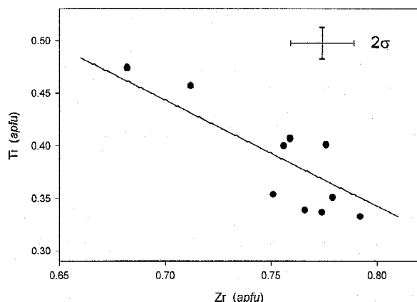
FIGURE 2. Variation in Ti as a function of Zr content in the sogdianite crystal analyzed here. The solid line was drawn by eye with a slope of 1.0, corresponding to Ti 4+ Zr substitution with Fe 3+ and Al constant.
